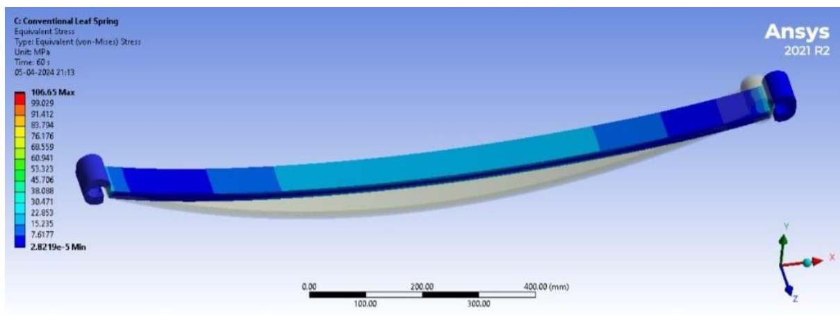
Von-Mises stress under static load of Composite leaf spring
