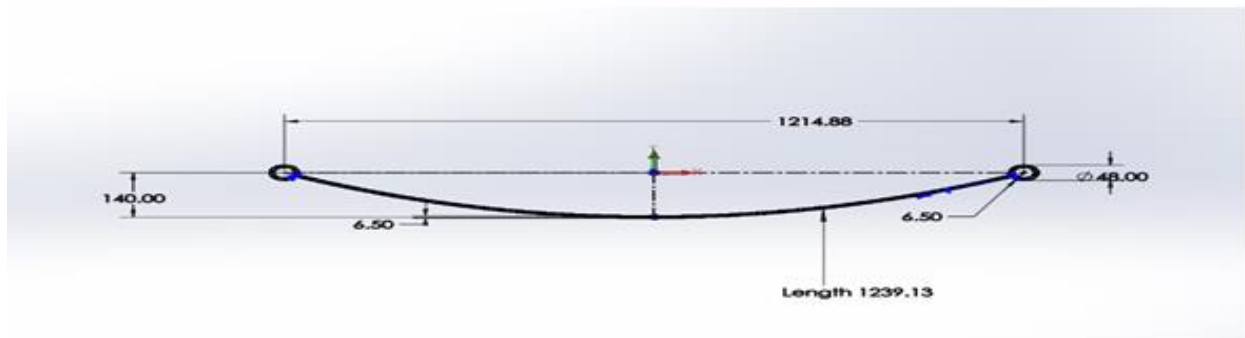
Figure.4 Design of leaf spring
