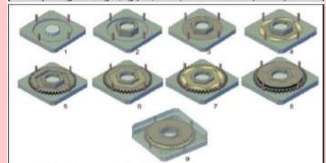
Figure 2. Hybrid gear assembly process.
